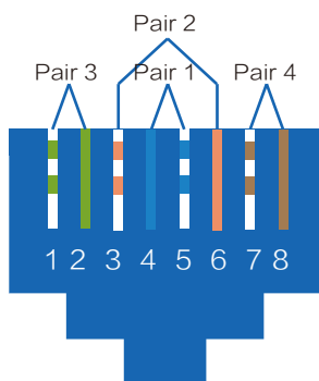
EIA T568A
