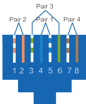
EIA T568B
