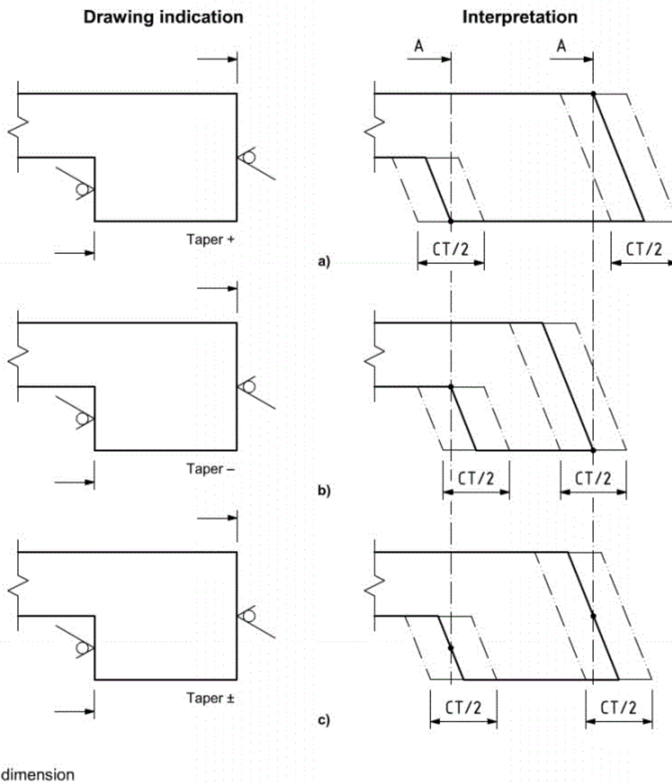
Figure B.1 — Tolerance zone on tapered features
