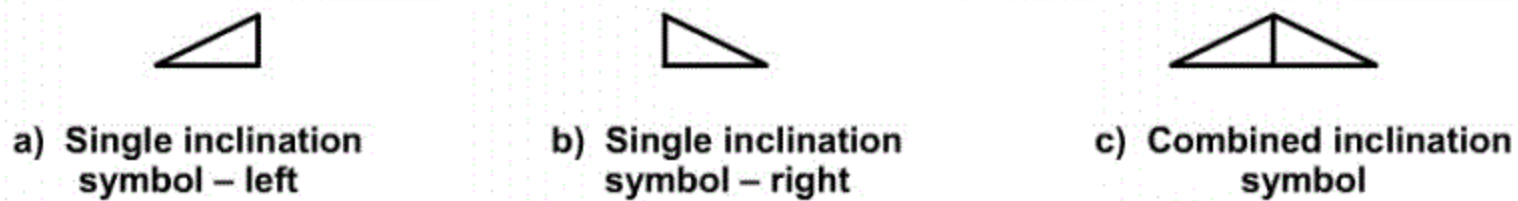
Figure 61 — Graphical symbol for representing draft angles
