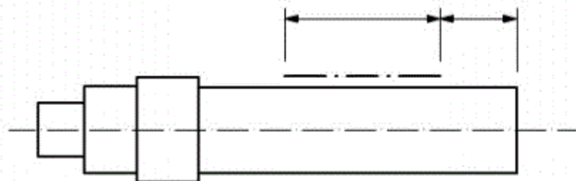
Figure 37 — Indication of restricted area of a feature
