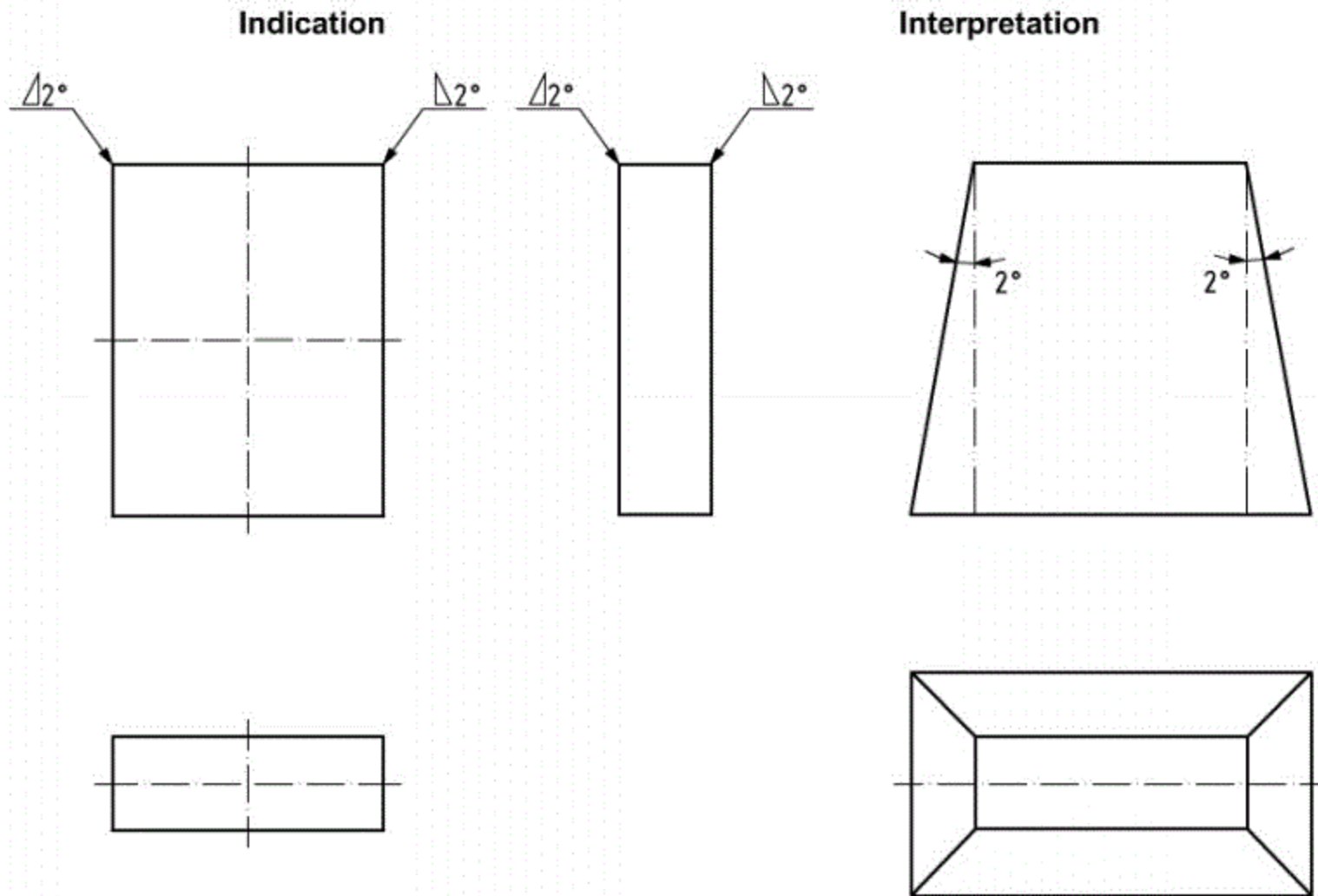
Figure 76 — Individual draft angle indication on four features
