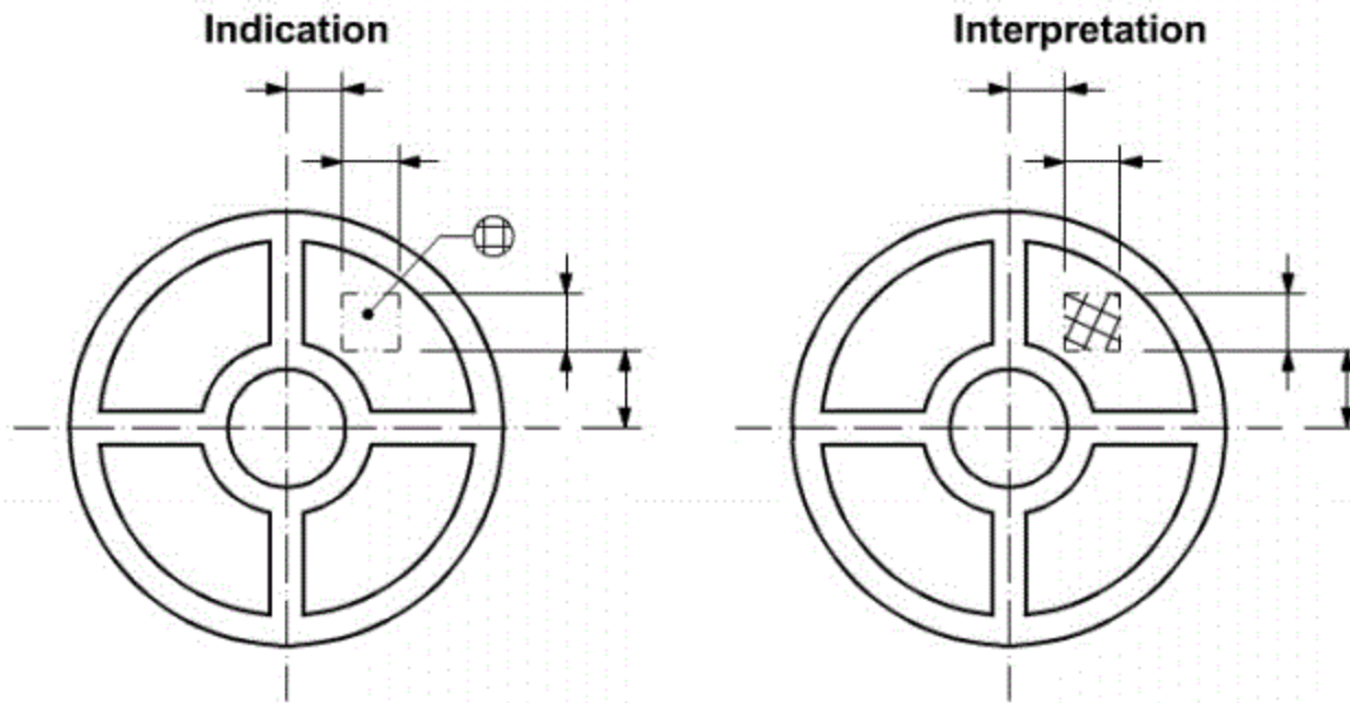
Figure 96 — Example of surface enlargement
