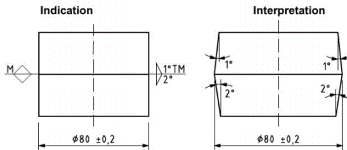
Figure 68 — Combined inclination with subtracted taper (TM)
