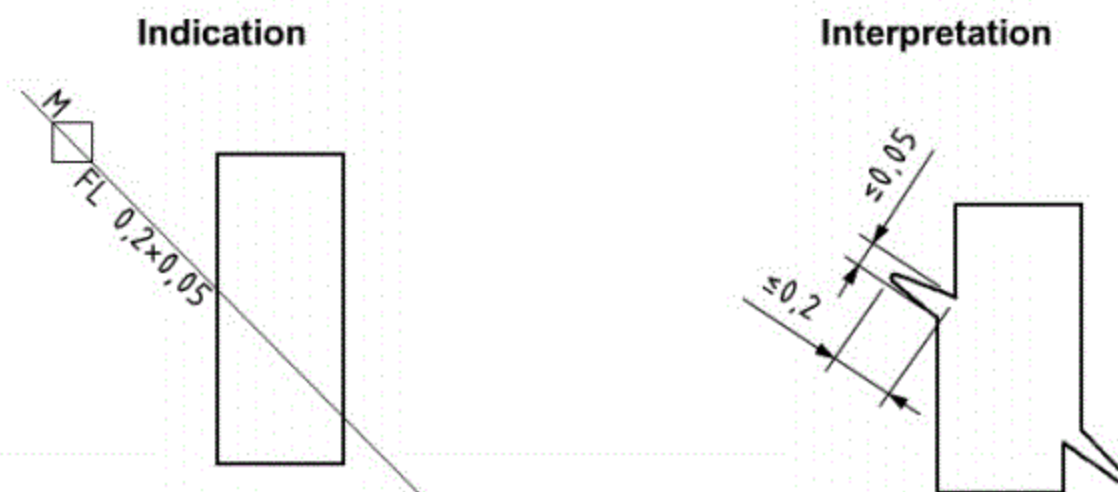
Figure 29 — Example of the interpretation of flash requirement
