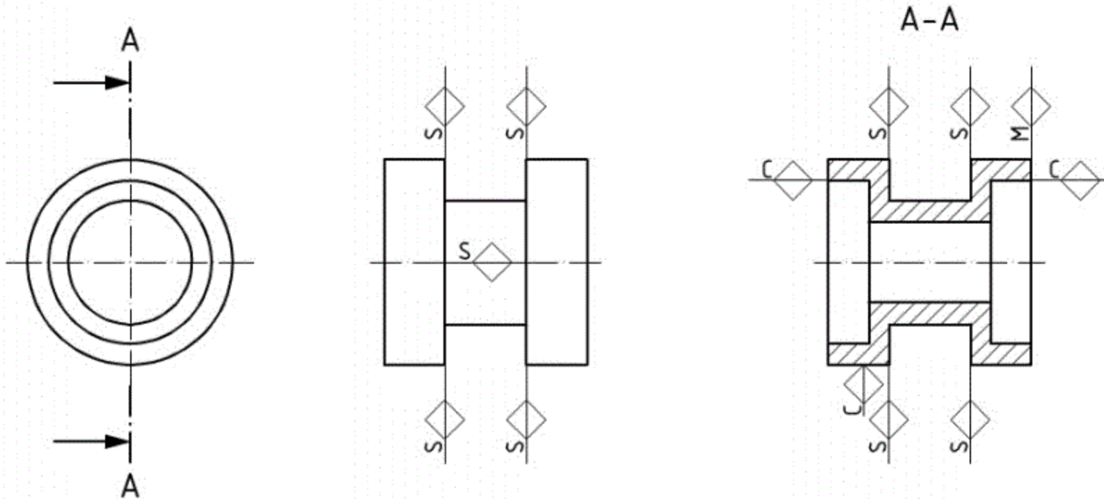
Figure 4 — Examples of the indication of parting surfaces
