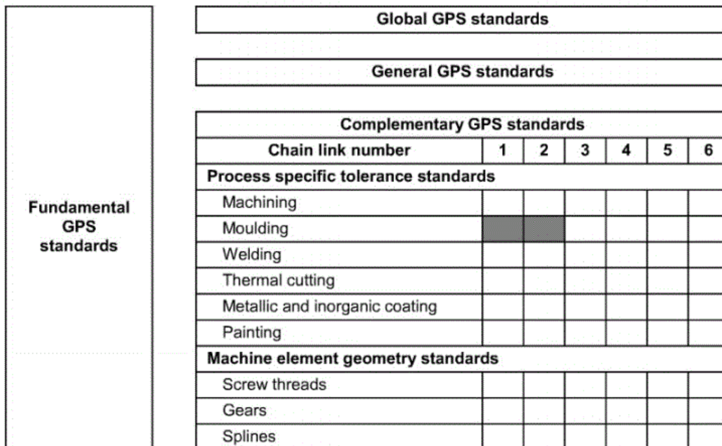
Figure C.1 — Position in the GPS matrix model
