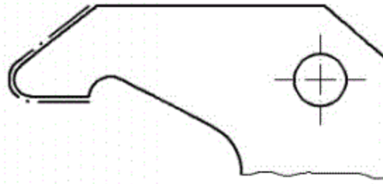
Figure 38 — Indication of a combination of adjoined features
