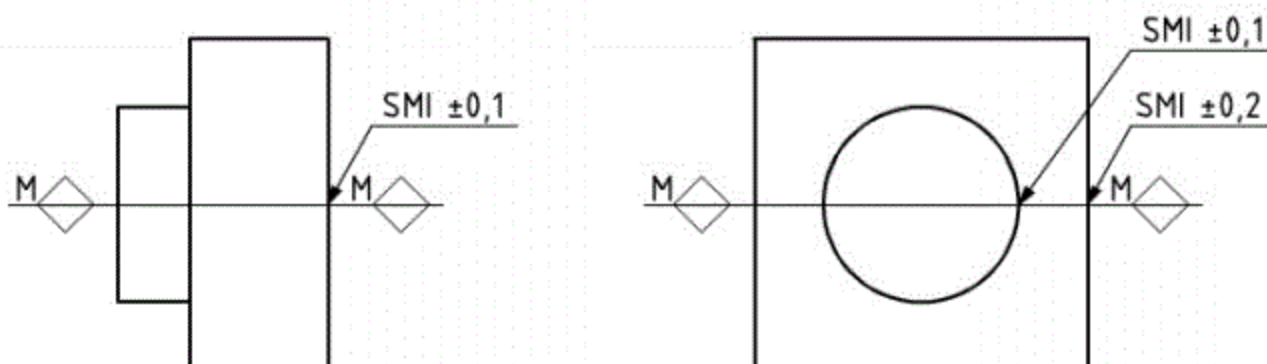
Figure 25 — Example of surface mismatch at individual features
