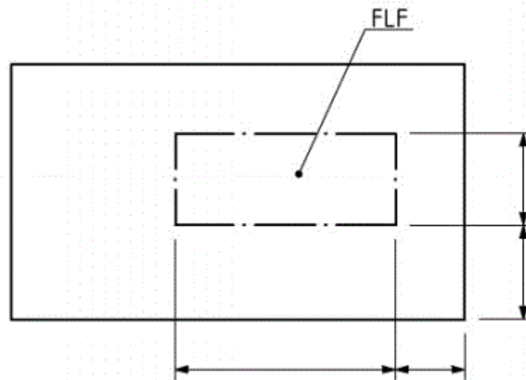
Figure 40 — Indication of flash-free area on a restricted area of a feature (plan)
