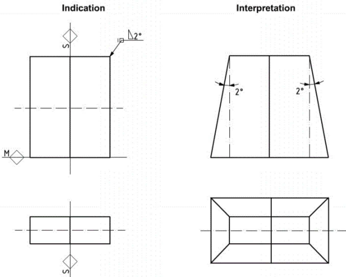
Figure 76 — Individual draft angle indication on four features
