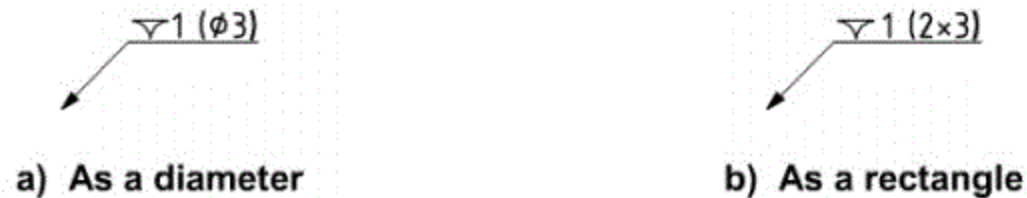
Figure 100 — Example of sink marking symbol used with maximum permissible dimension of sink mark
