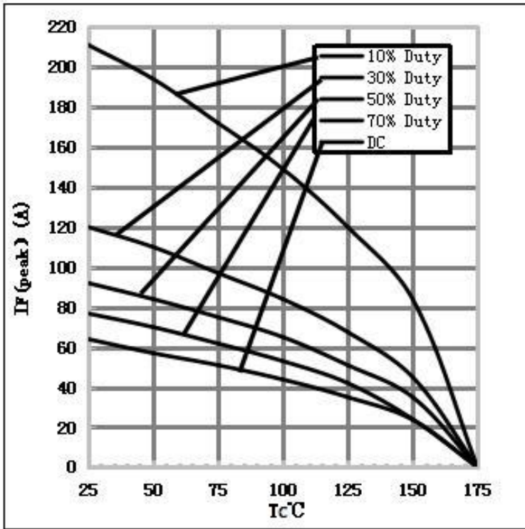
3) 不同负载下的电流 (Current Derating) (10%, 30%, 50%, 70%, DC)
