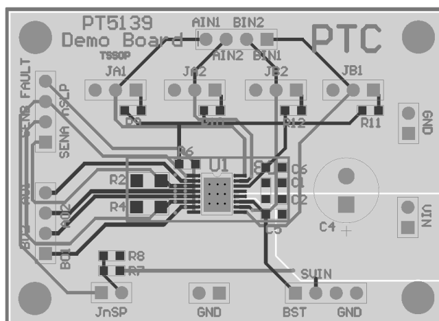
Figure 8: TSSOP-16
