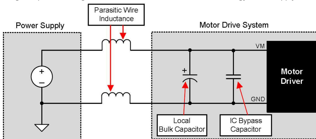
Figure 6 : Example Setup of Motor Drive System with External Power Supply
