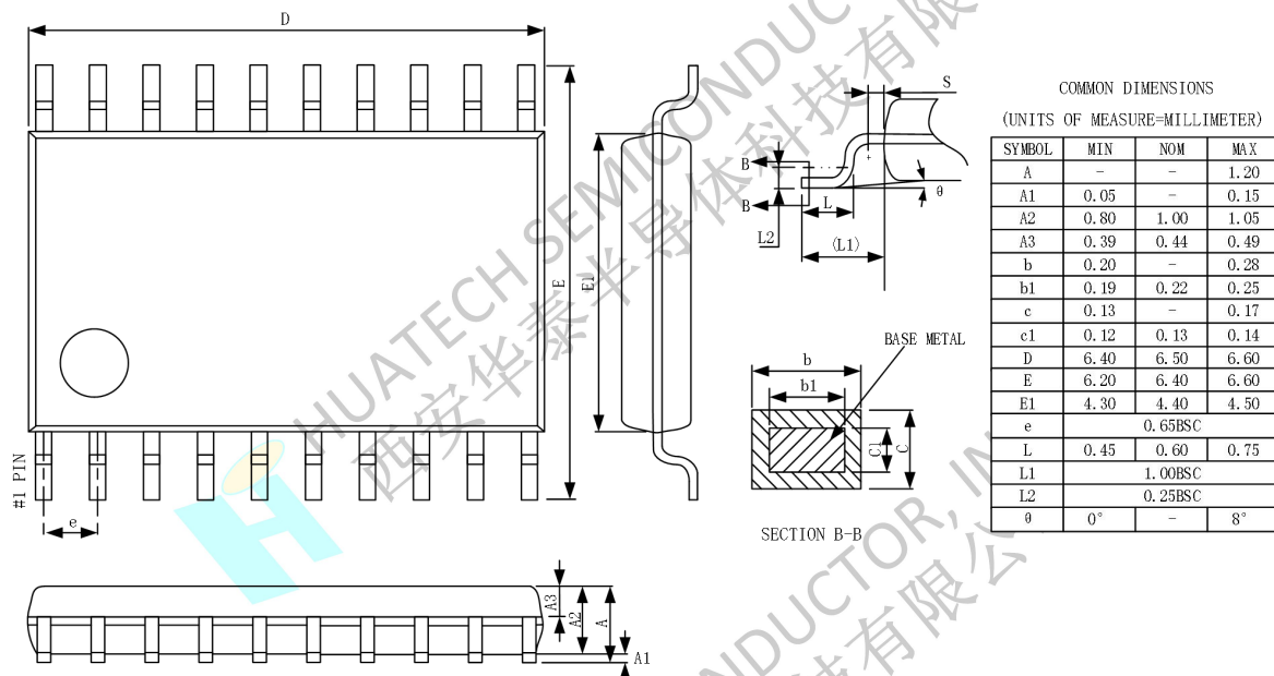
20-Lead TSSOP Package Outline Diagram
