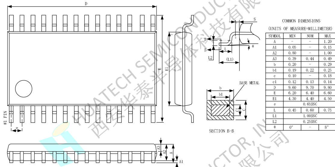
28-Lead TSSOP Package Outline Diagram
