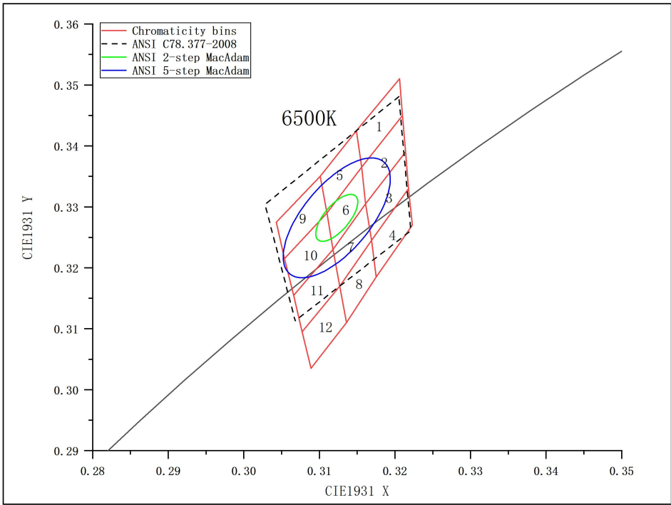
不同 BIN 号对应标签色温与色温范围。 Different BIN number correspond to the CCT and CCT range .
