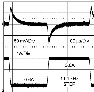
Figure 13. Transient Response
