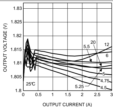
Figure 11. Line and Load Regulation at 25°C
