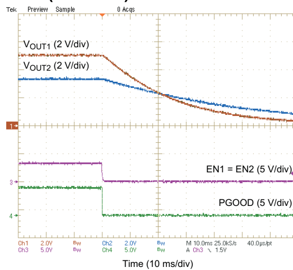
Figure 24. Output Discharge
