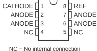
TL431, TL431A, TL431B ... D (SOIC) PACKAGE (TOP VIEW)
