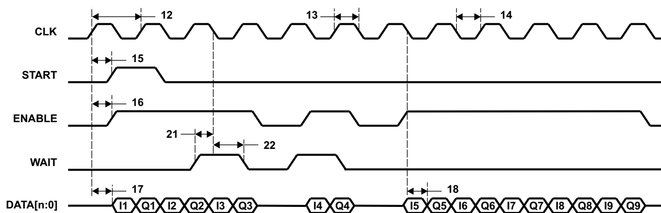
Figure 7-82. uPP Double Data Rate (DDR) Transmit Timing
