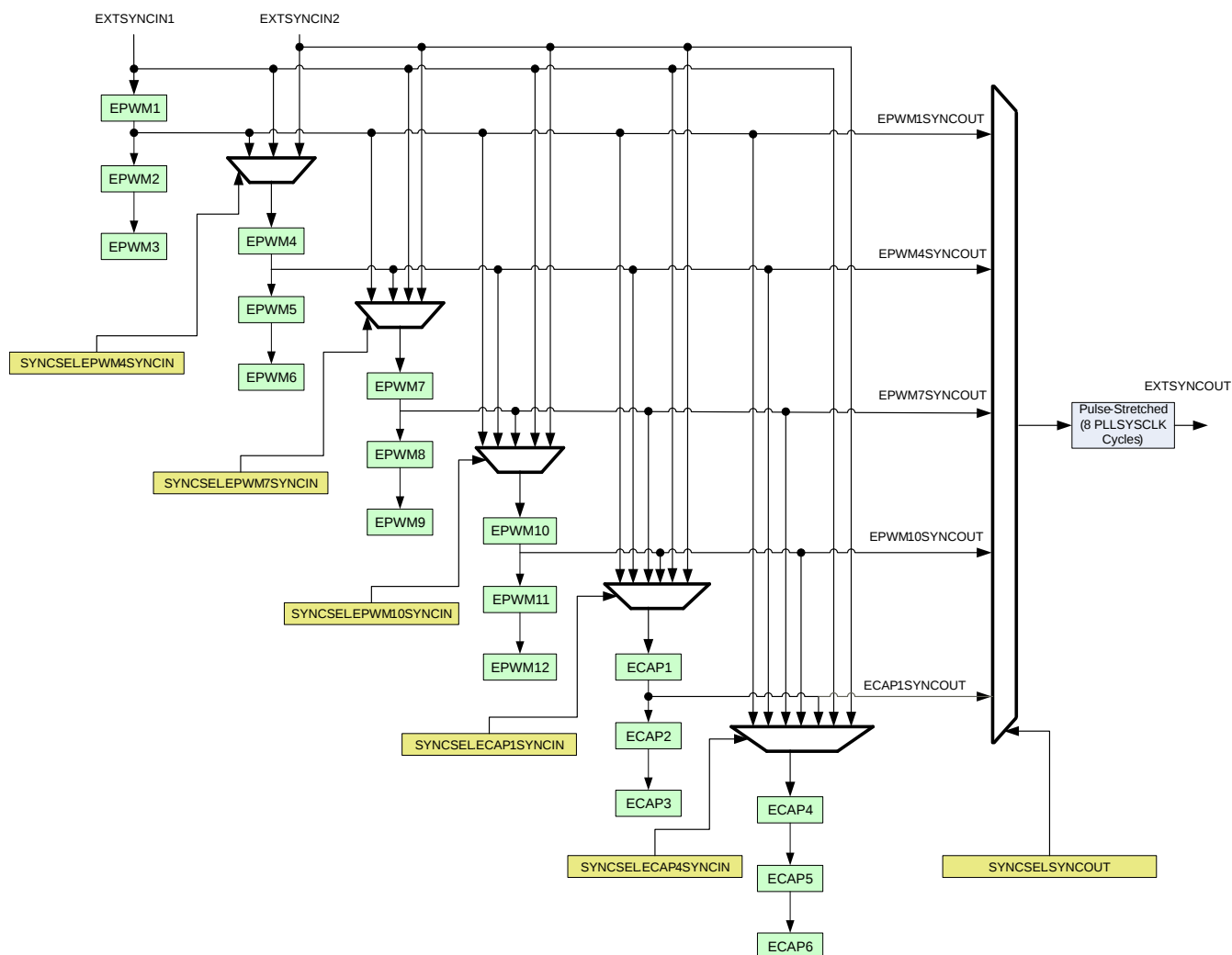
Figure 7-51. Synchronization Chain Architecture
