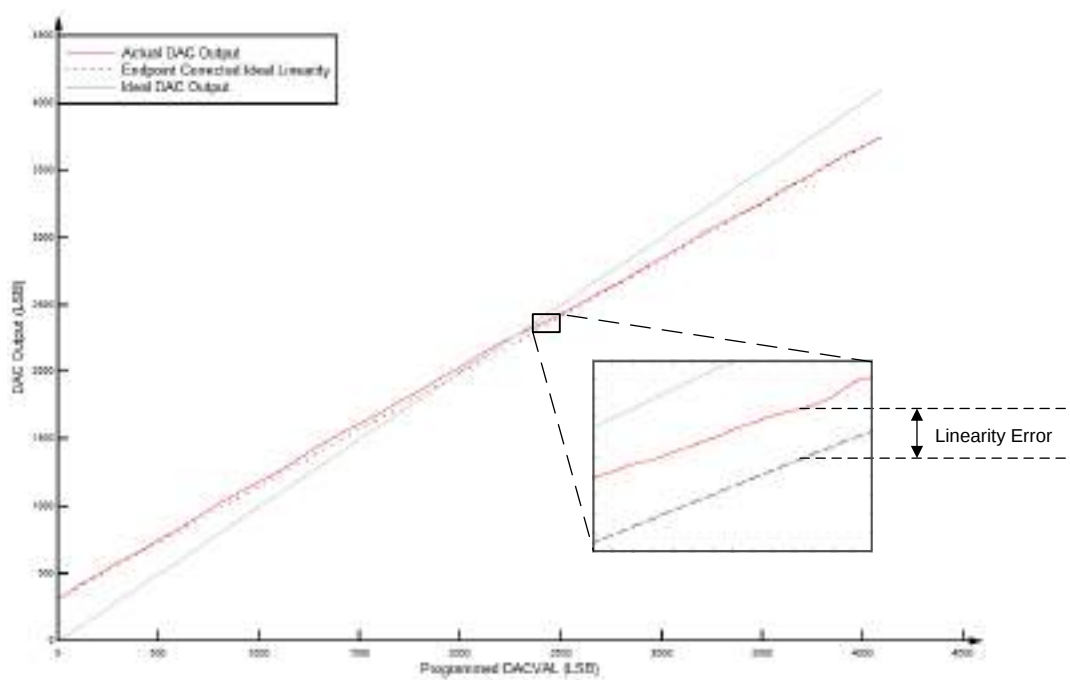
Figure 7-43. CMPSS DAC Static Linearity
