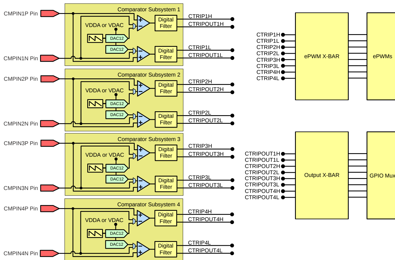
Figure 7-38. CMPSS Connectivity (100-Pin PZP)
