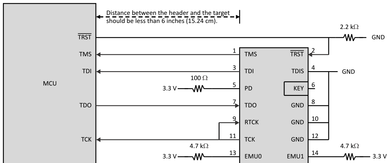
Figure 7-9. Connecting to the 14-Pin JTAG Header
