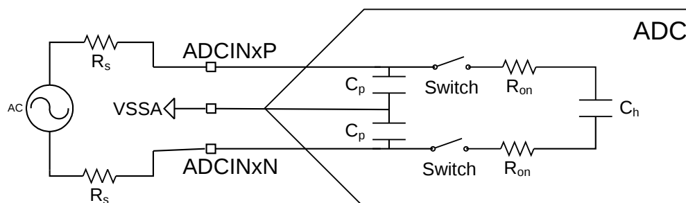
Figure 7-33. Differential Input Model
