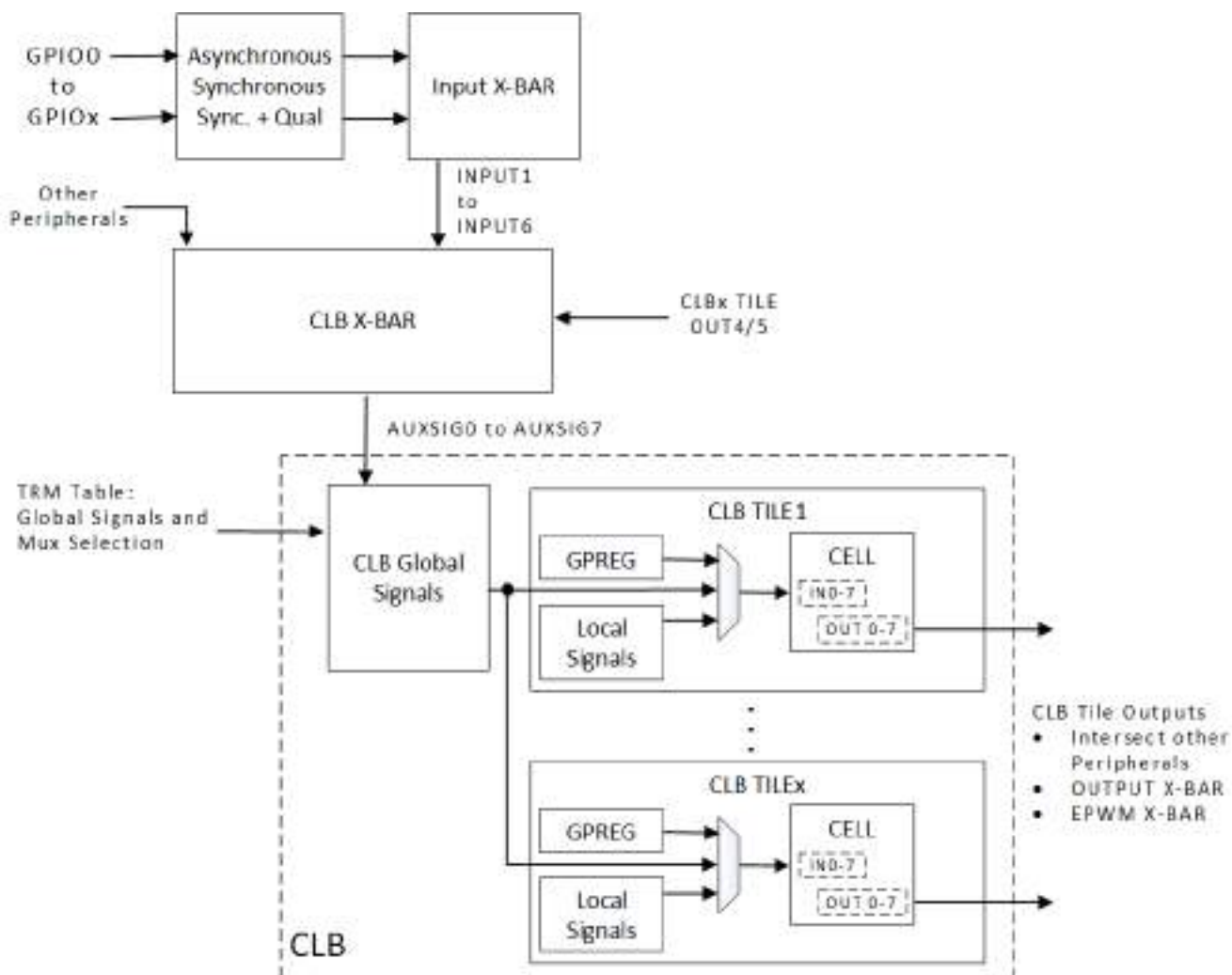
Figure 8-5. CLB Overview
