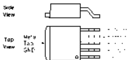
图 6-2. 5-Pin TO-263 KTT Package Top View
