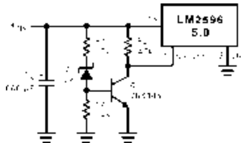
图 8-2. Undervoltage Lockout for Buck Regulator
