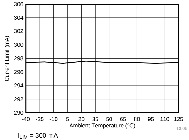
图 8. Current Limit vs Ambient Temperature
