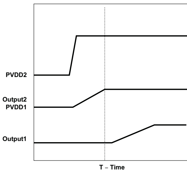
Figure 35. Waveforms Resulting from Cascading PVDD1 from Output 2
