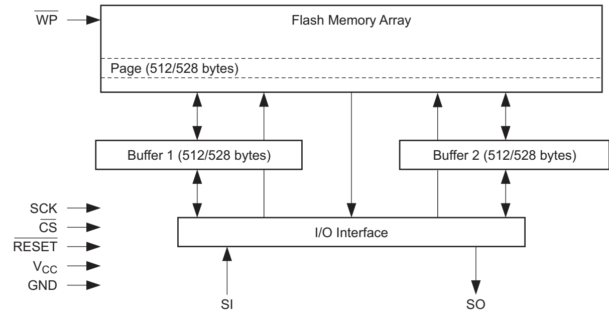
Figure 2-1. Block Diagram
