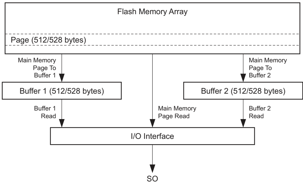
Figure 23-1. Block Diagram
