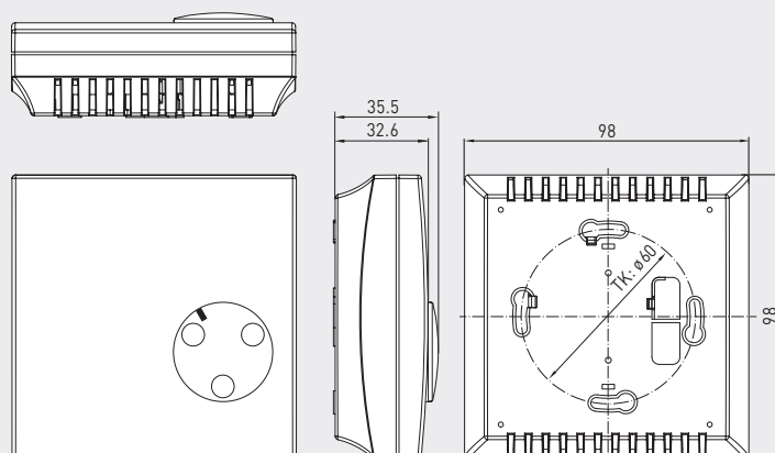
Housing Baldur 2 RH-2
