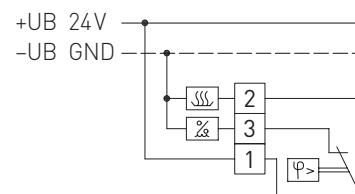
Connecting diagram
