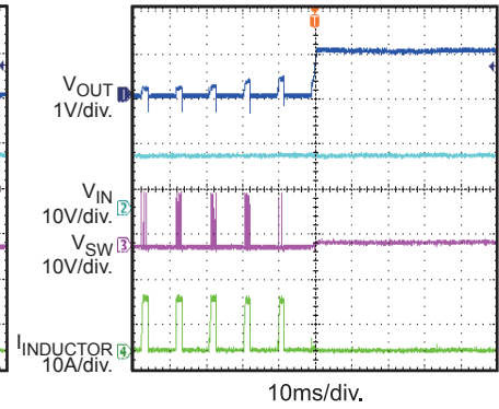
Short-Circuit Recovery
