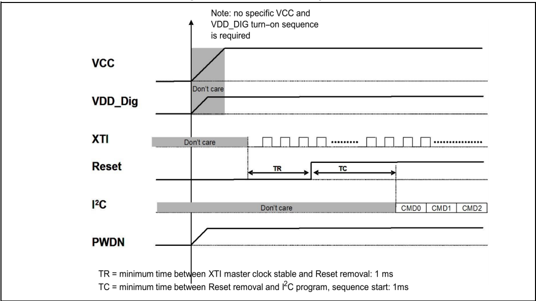
Figure 4. Power-on sequence
