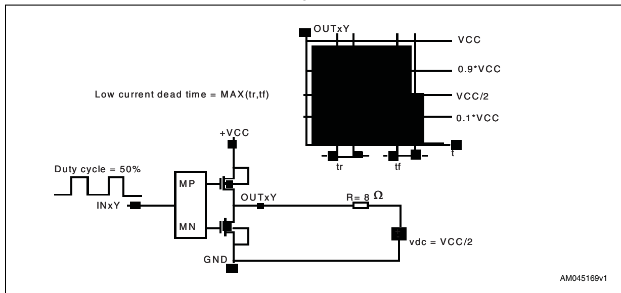
Figure 3. Test circuit
