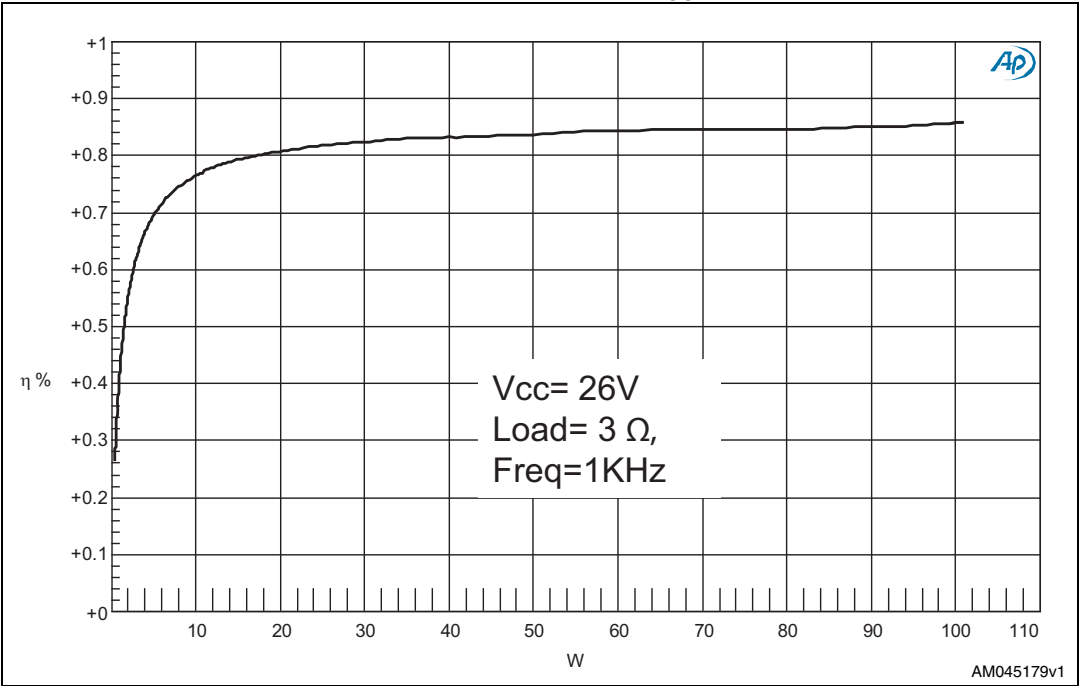
Figure 16. Efficiency vs. output power ( V_{CC} = 26\text{ V} , load = 3\ \Omega )
