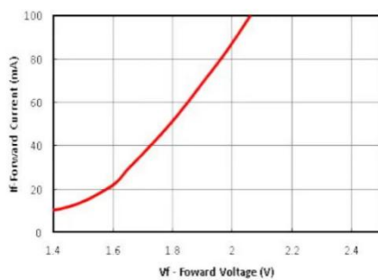
I-V Graph
