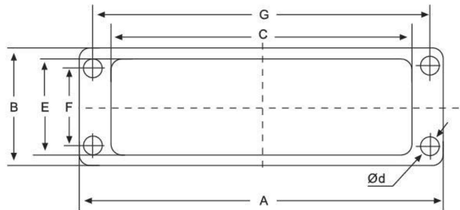
H10A,H16A,H32A开孔底座; H6B,H10B,H16B,H24B,H32B,H48B开孔底座
