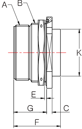
Mounting dimensions
