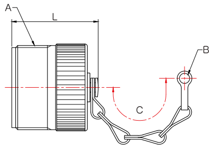
JW17350(MS17350) plug protective cover
