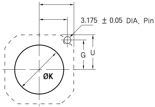
Mounting dimensions
