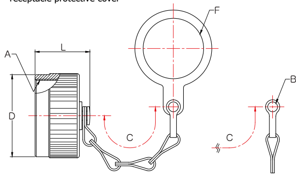
JW17349A/B(MS17349A/B) receptacle protective cover
