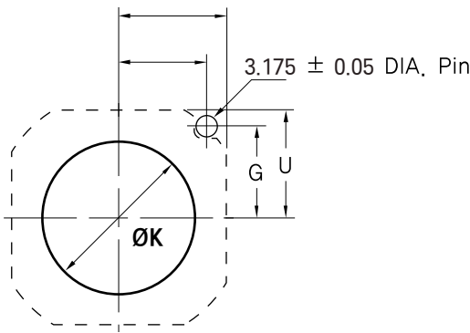
Mounting dimensions
