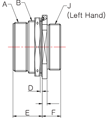
Mounting dimensions
