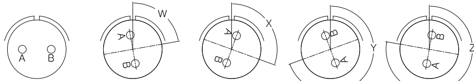
NORMAL POSITION POSITION "W" POSITION "X" POSITION "Y" POSITION "Z"
