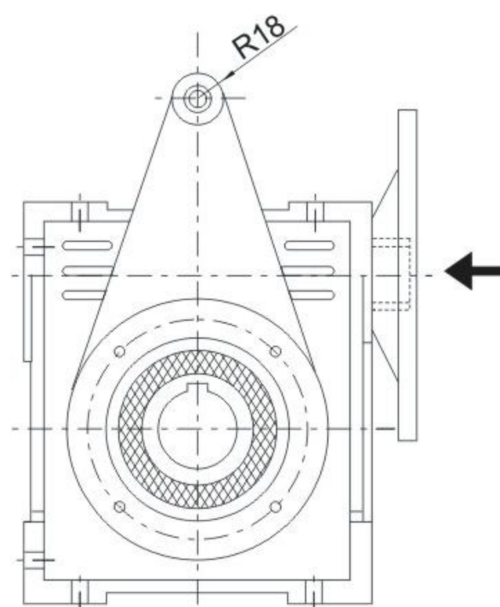
NMRV040.....SZ
