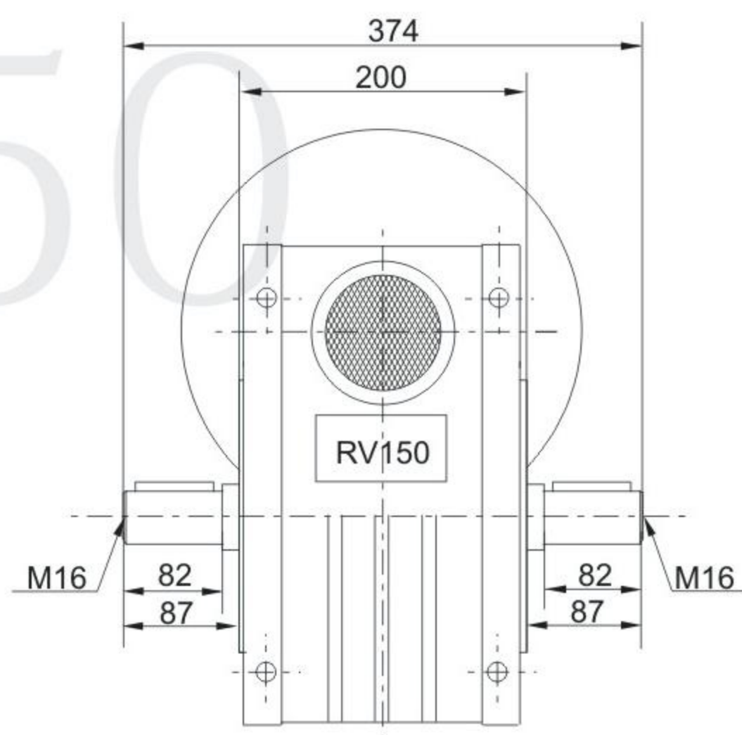
NMRV150.....SZ
