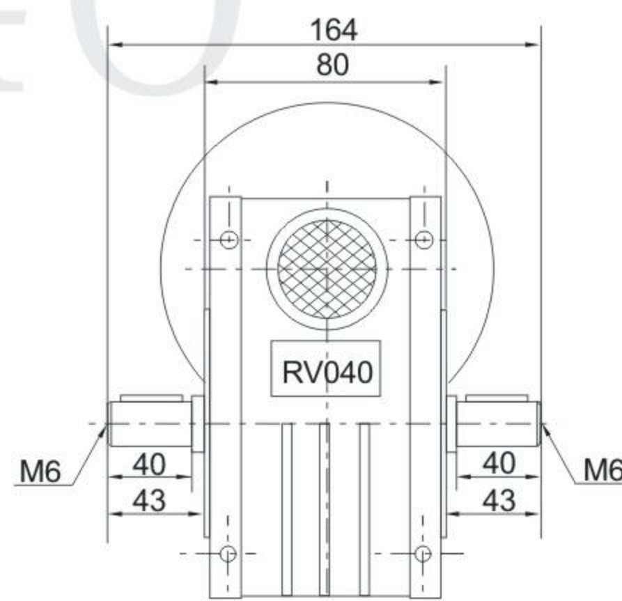
NMRV040.....SZ
