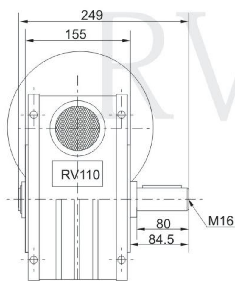
NMRV110.....DZ
