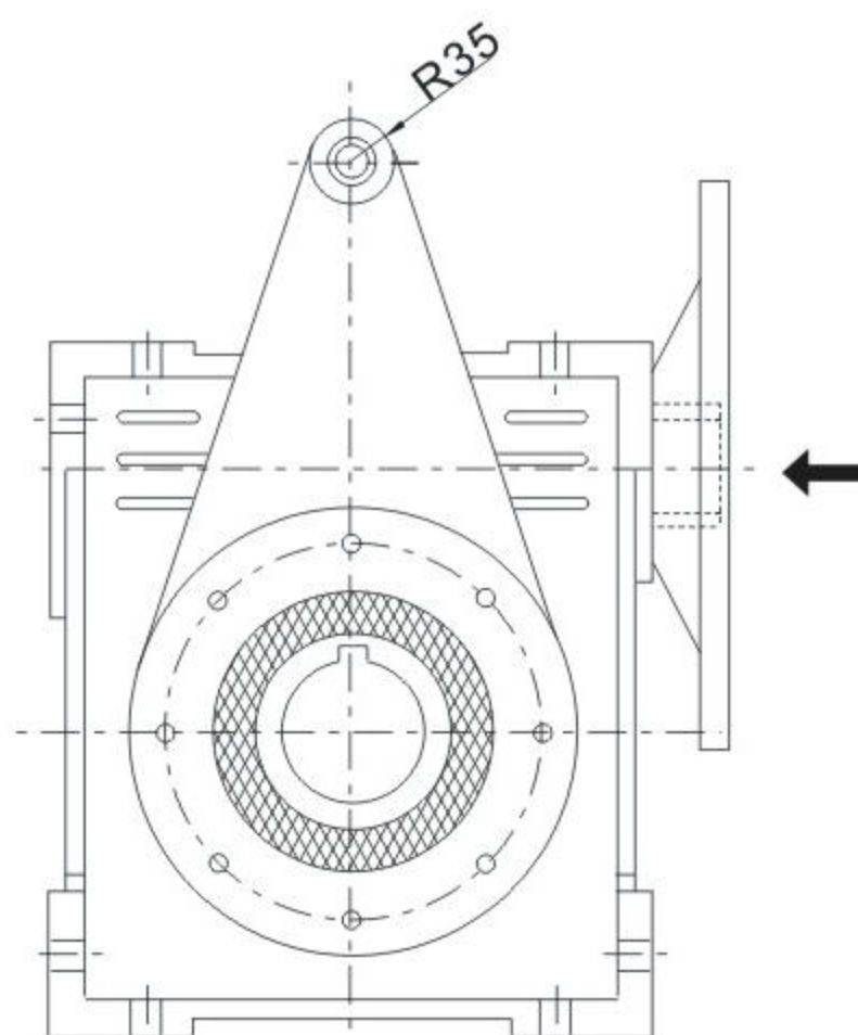
NMRV150.....TA
