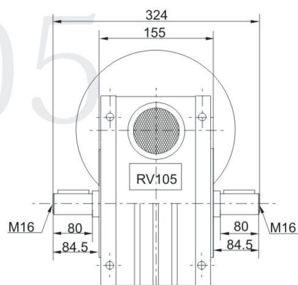
NMRV105.....SZ
