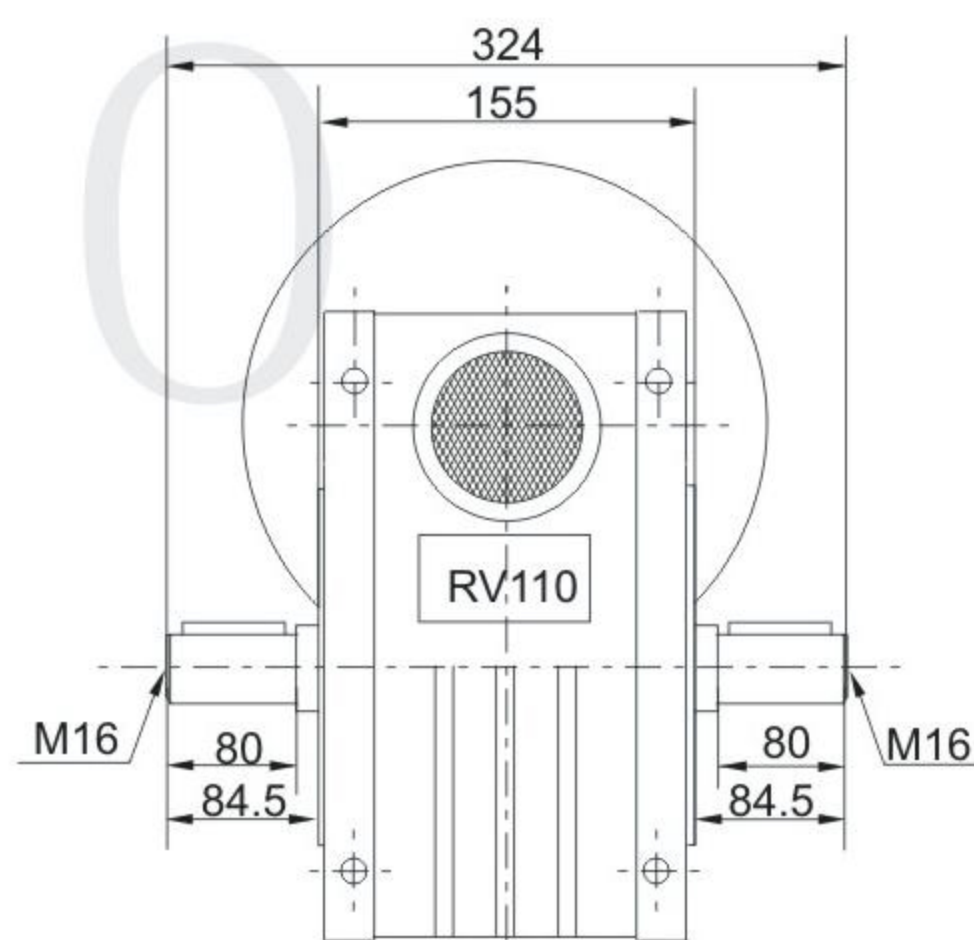
NMRV110.....SZ
