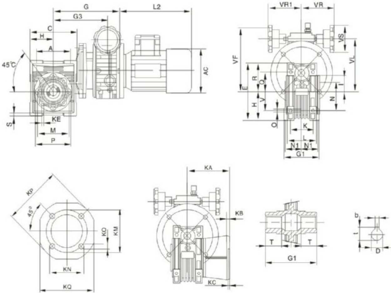
外型及安装尺寸 Outline & installation sizes
