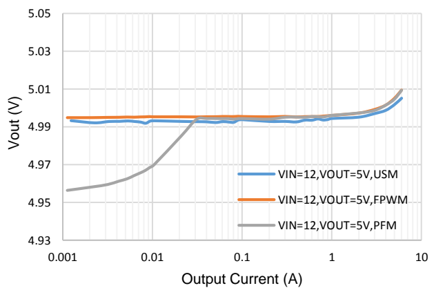
Figure 7. Load Regulation, Vout=5V, fsw=800kHz
