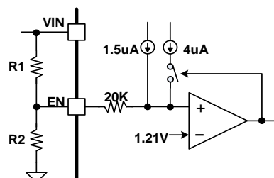
Figure 9. System UVLO by enable divide
