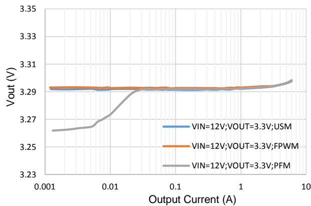
Figure 6. Load Regulation, Vout=3.3V, fsw=800kHz
