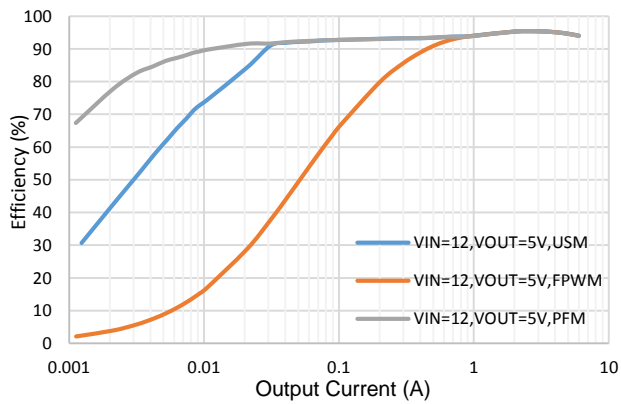
Figure 4. Efficiency vs Iload, Vout=5V, fsw=800kHz
