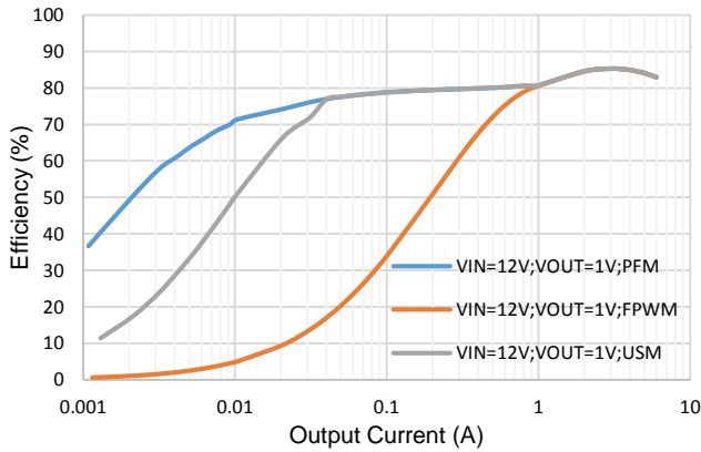
Figure 2. Efficiency vs Iload, Vout=1V, fsw=800kHz
