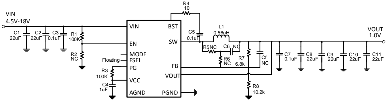
Figure 10. SCT2260A Design Example, 1V Output
