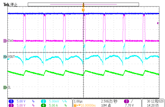
Figure 21. Output Ripple (Iload=6A)
