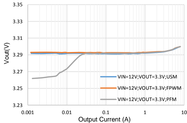
Figure 6. Load Regulation, Vout=3.3V, fsw=800kHz
