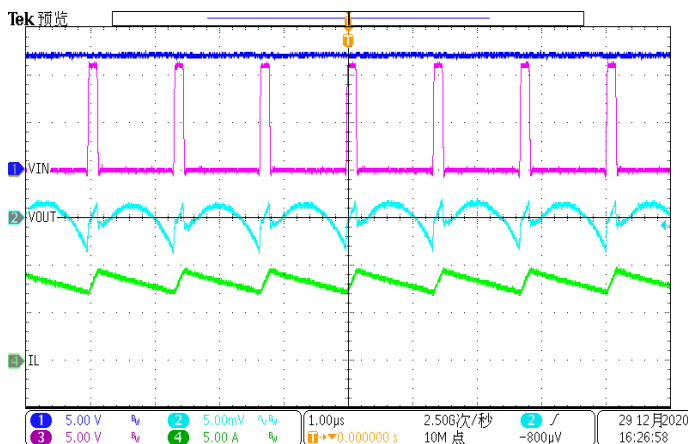
Figure 21. Output Ripple (Iload=8A)
