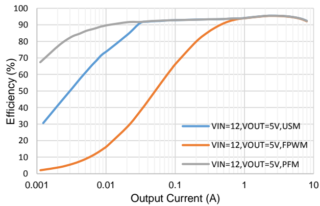
Figure 4. Efficiency vs Iload, Vout=5V, fsw=800kHz
