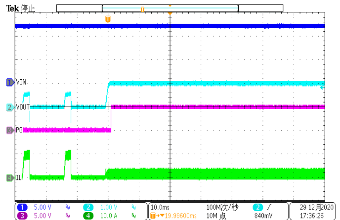
Figure 16. Over Current Release (hard short to 1A)
