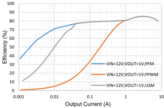
Figure 2. Efficiency vs Iload, Vout=1V, fsw=800kHz
