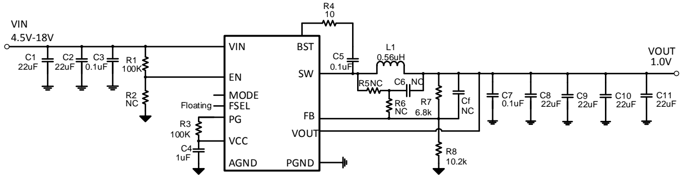
Figure 10. SCT2280 Design Example, 1V Output
