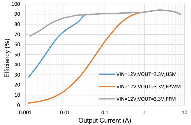
Figure 3. Efficiency vs Iload, Vout=3.3V, fsw=800kHz
