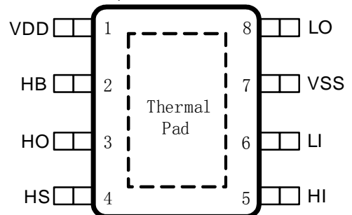
Top View: ESOP-8L
