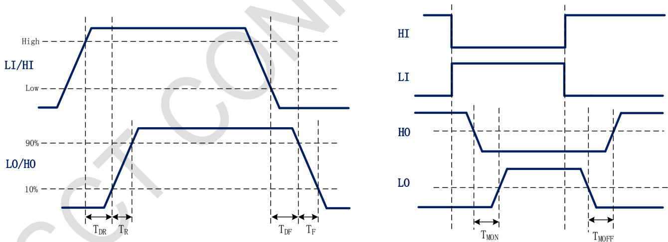
Figure 1. Timing Diagram
