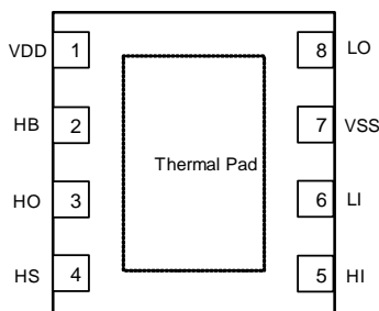
Top View: DFN-8L(4mm*4mm)
