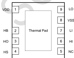
Top View: DFN-9L(3mm*3mm)
