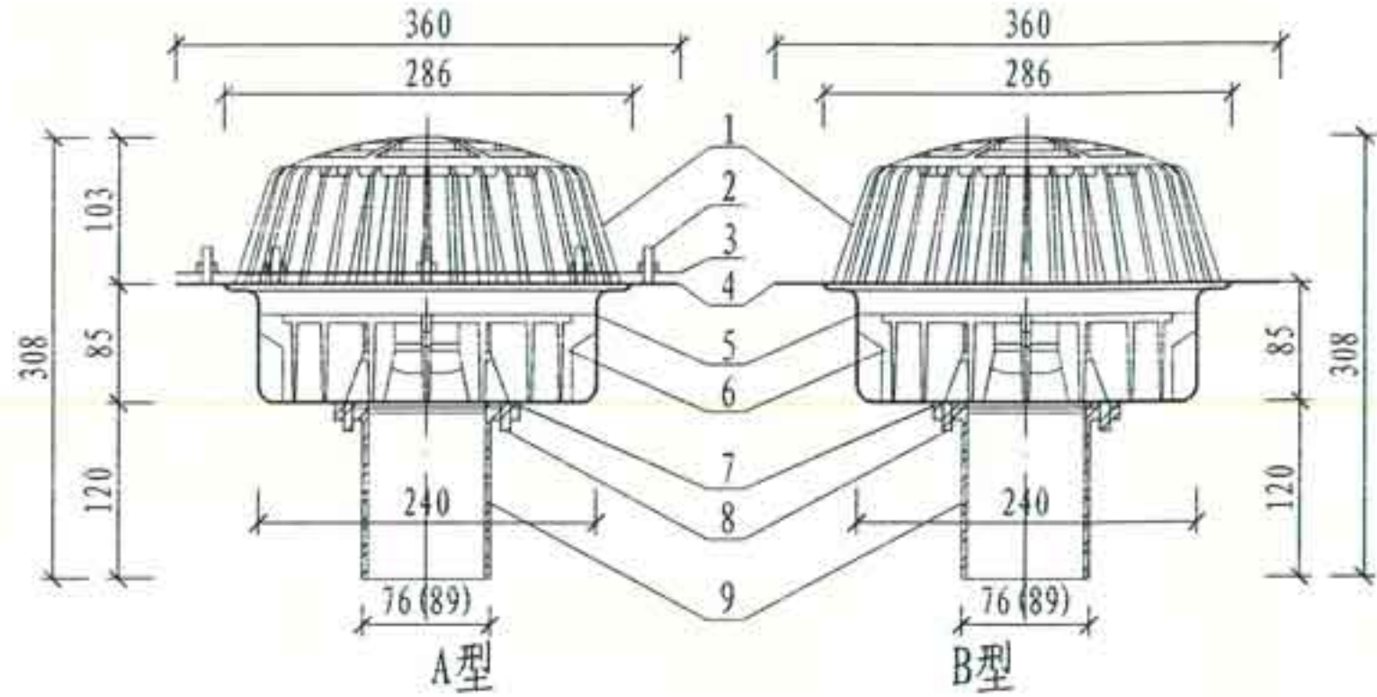
② YG75 (80)型虹吸式雨水斗
