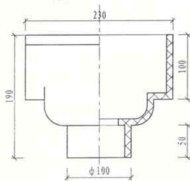
③ UPVC方雨水斗
