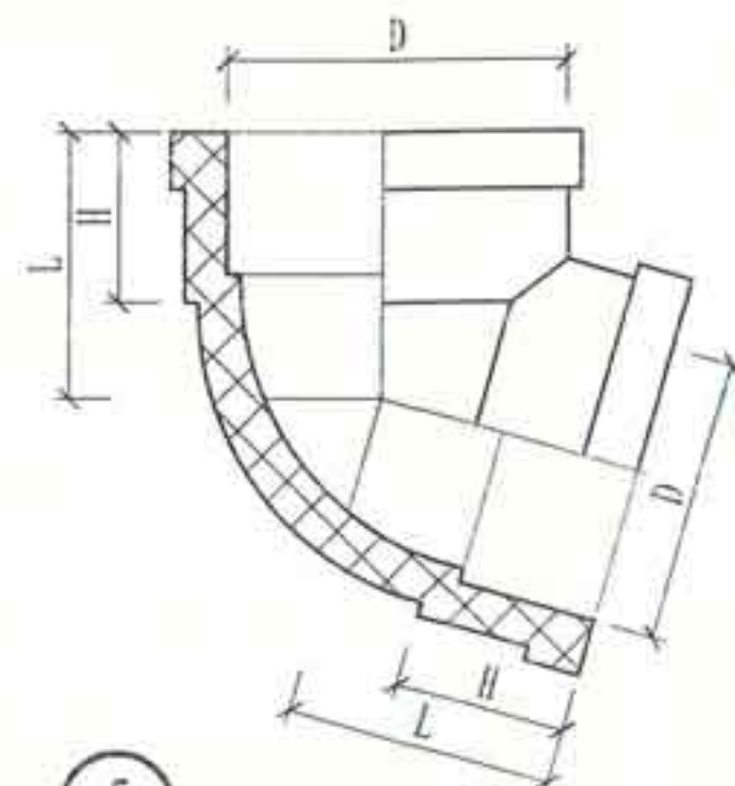
UPVC45°弯头透视
